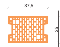
Porotherm 25/37.5 AKU
