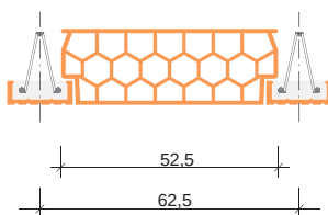
stropy Porotherm 62,5
